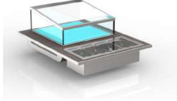
Ice Bin Module with Condiment Holder (1/3)
