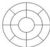
Ø5490 x 760 mm WM-DE-BTSSC05 2873 (L) x 915 (W) x 760 (H) mm 2154 (L) x 915 (W) x 760 (H) mm Outer Ø: 5490 mm Inner Ø: 1830 mm
